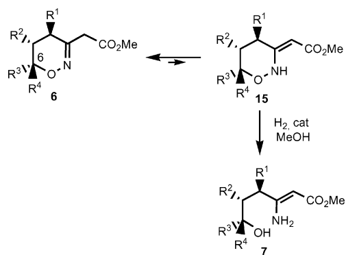
Scheme 9. Possible route to enamines 7 from dihydrooxazines 6 .
