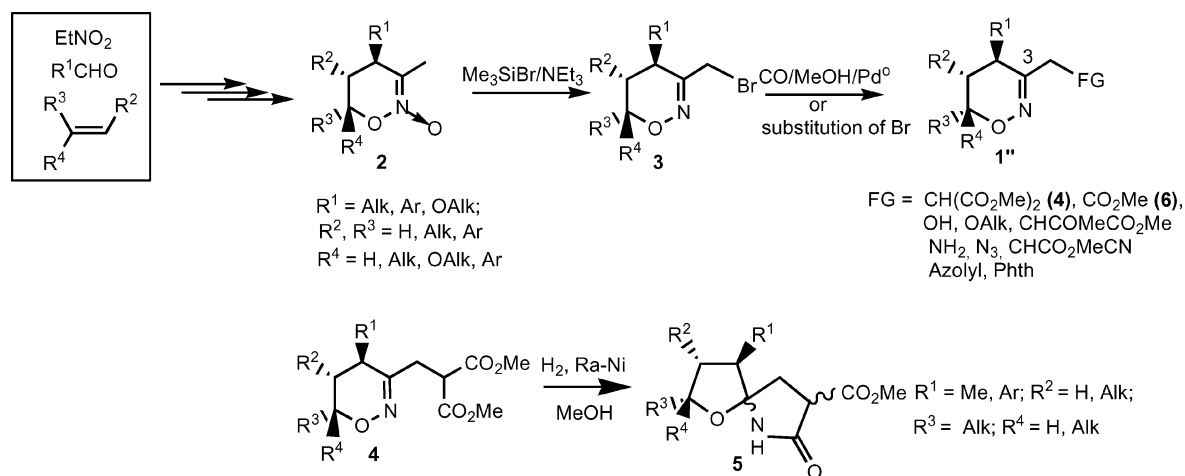
Scheme 2. Synthesis and hydrogenation of 5,6-dihydro-4H-1,2-oxazines with a functionalized methylene group at C-3.
