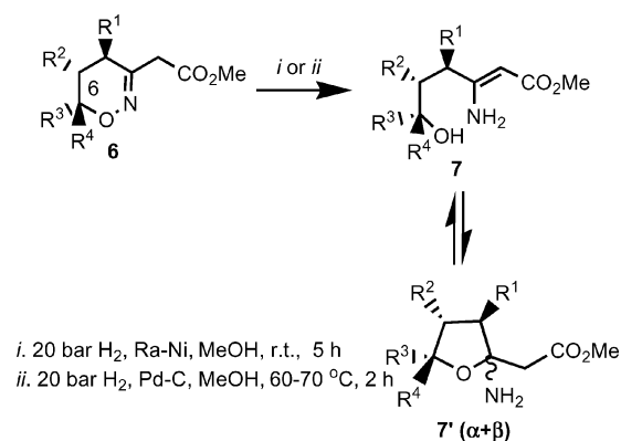
Scheme 3. Hydrogenation of dihydrooxazines 6 to enamines 7 .
