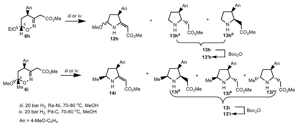
Scheme 6. Catalytic hydrogenation of dihydrooxazines 6h,i .
