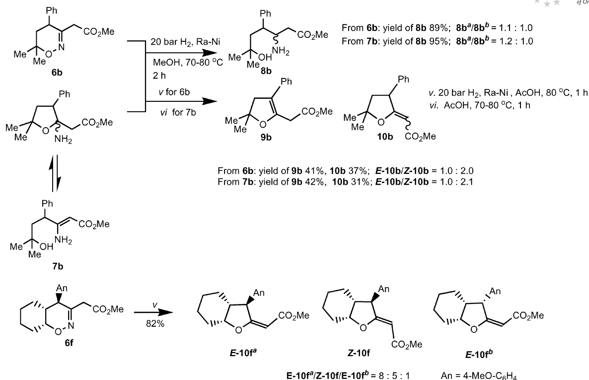
Scheme 4. Comparison of the catalytic hydrogenation of oxazines 6b and 6f with the hydrogenation of enamine 7b .
