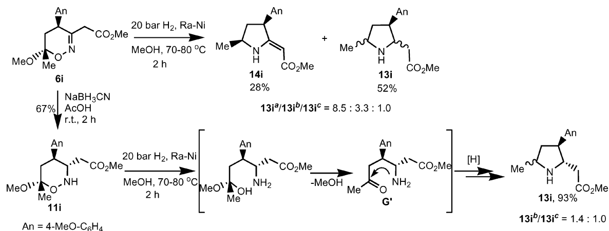
Scheme 10. Comparison of the hydrogenation reactions of oxazine 6i and tetrahydrooxazine 11i .
