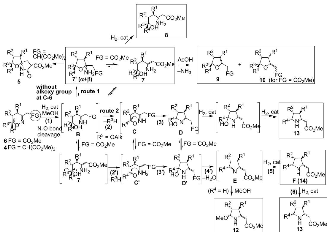
Scheme 8. General mechanistic scheme for the catalytic hydrogenation of 5,6-dihydro-4 H -1,2-oxazines bearing a functionalized methylene group at C-3.
