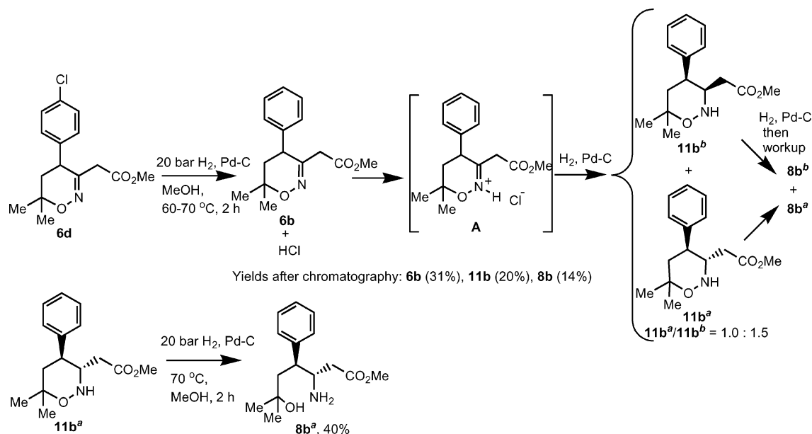
Scheme 5. Hydrogenation of dihydrooxazine 6d in the presence of Pd-C.
