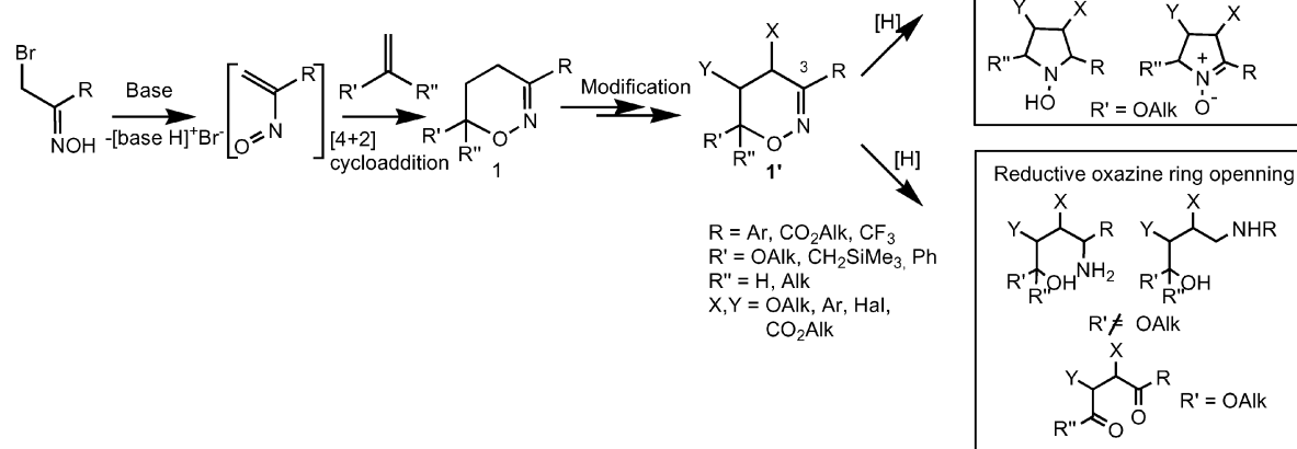
Scheme 1. 5,6-Dihydro-4 H -1,2-oxazines in organic synthesis.
