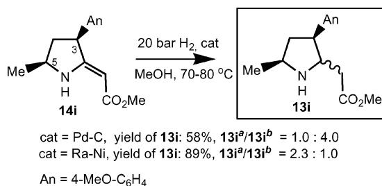
Scheme 7. Catalytic hydrogenation of enamine 14i .
