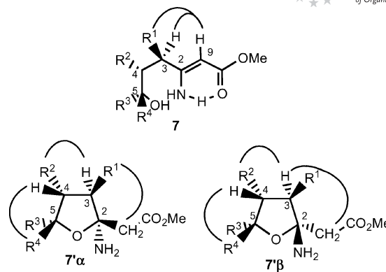
Figure 1. Characteristic 2D NOESY correlations in 7 and 7' .
