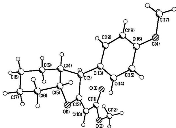
Figure 2. X-ray crystal structure of compound E-10f a recorded at 293(2) K.
